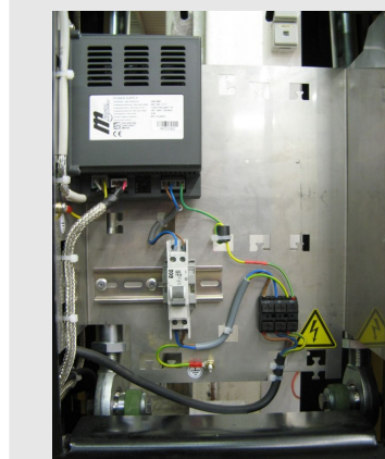
mounting panel
