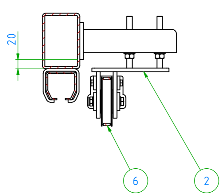
C-C (1:5)
