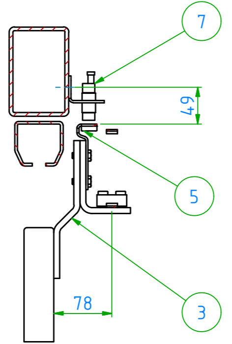
B-B (1:5)
